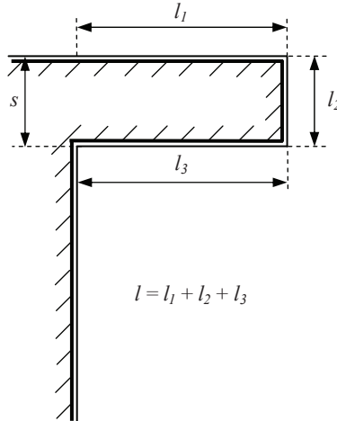
Fig. 6.24 – Bucla unui conductor de coborâre
